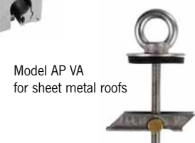
Model AP VA for seam roofs
